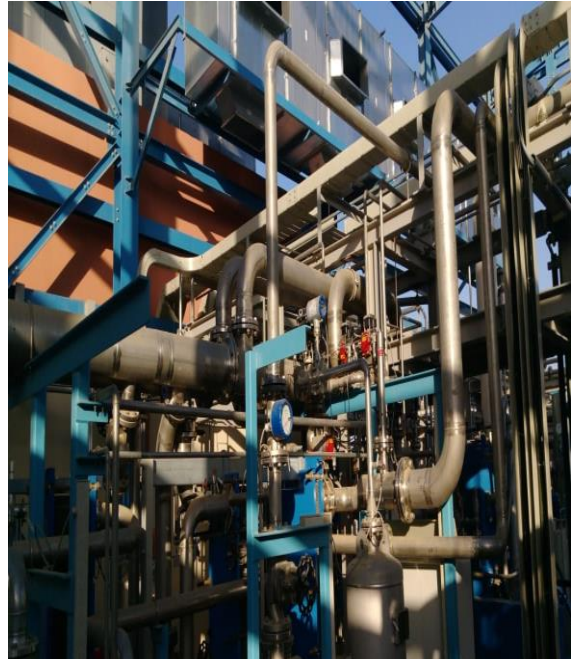
Co2 Piping / Structural Works – Shuaibah III Expn II Diesel Plant (2019)
