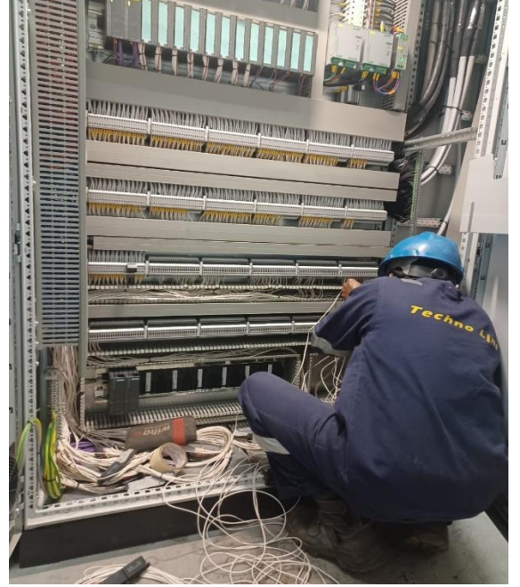
Electrical Panel Termination Works – ILMENITE SMELTING PLANT AMIC – JAZAN (2021)
