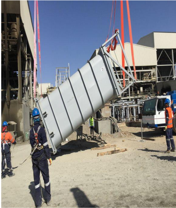
Upgradation of Flotation cells and Mill Enhancement, Phase-2 Modification, Ma'aden Goldmine, Al-Amar (2018)
