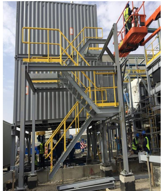
Installation of Pumps, Dosing units, Electrical and Instrumentation, Ma'aden Goldmine, Al-Amar (2017)
