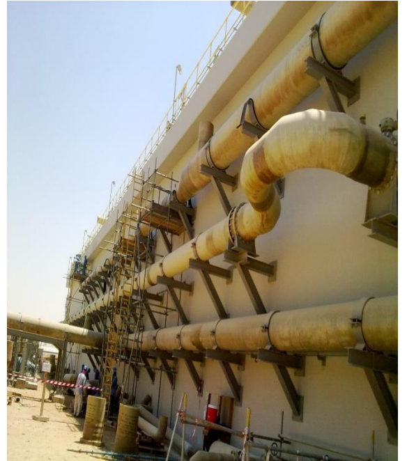
GRP Piping works – Marafiq /SETE IWTP-II Project Yanbu-2013
